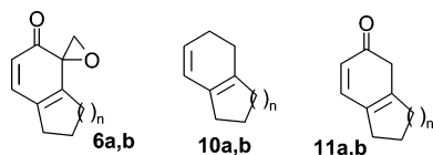
FIGURE 2. Cyclohexa-2,4-dienones and annulated cyclohexadiene.
