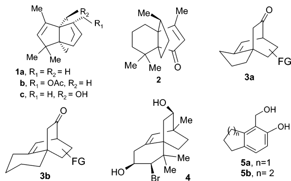
FIGURE 1. [3.3.3]- and [4.3.3]propellanes, tricyclic compound, sesquiterpene containing tricyclo[5.2.2.0 1,6 ]dodecane system, and aromatic precursor.
